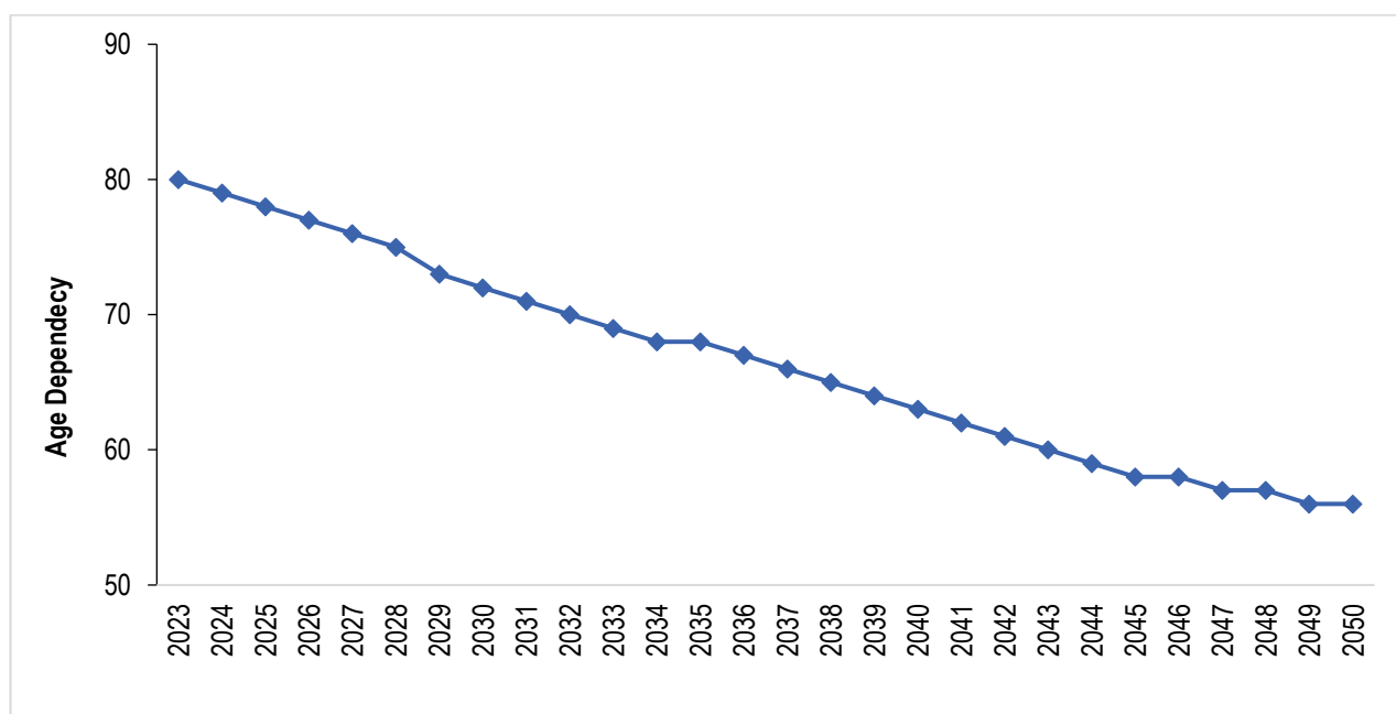
Figure 3. 4: Projected Age Dependency Ratio; Iringa Region, 2023 – 2050
